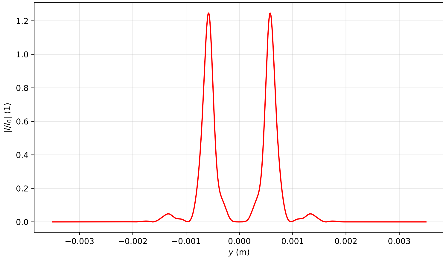
Intensity profile I(x=0, y, z=1.035)/I_0 , \text{Pin}=8.0\text{Pcr} , artificial time
